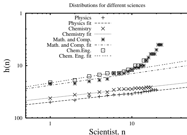
FIG. 1: The fits (1) for Physics, Chemistry, Mathematics plus Computer Science, and Chemical Engineering. For the two latter fields the entire data sets are shown as points, although the fits only include the k highest points in Table I.
